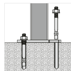
Floor mounting
