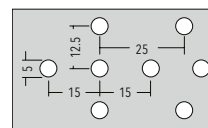
Euro hole pattern, dimensions in mm
