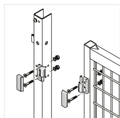
Top stop
