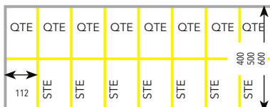
Sixteenth division, 7x STE and 8x QTE
