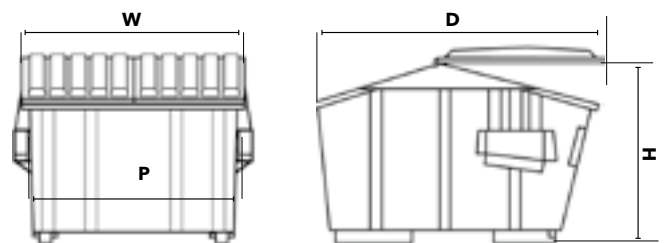
Front view and lateral view of the front loading container
